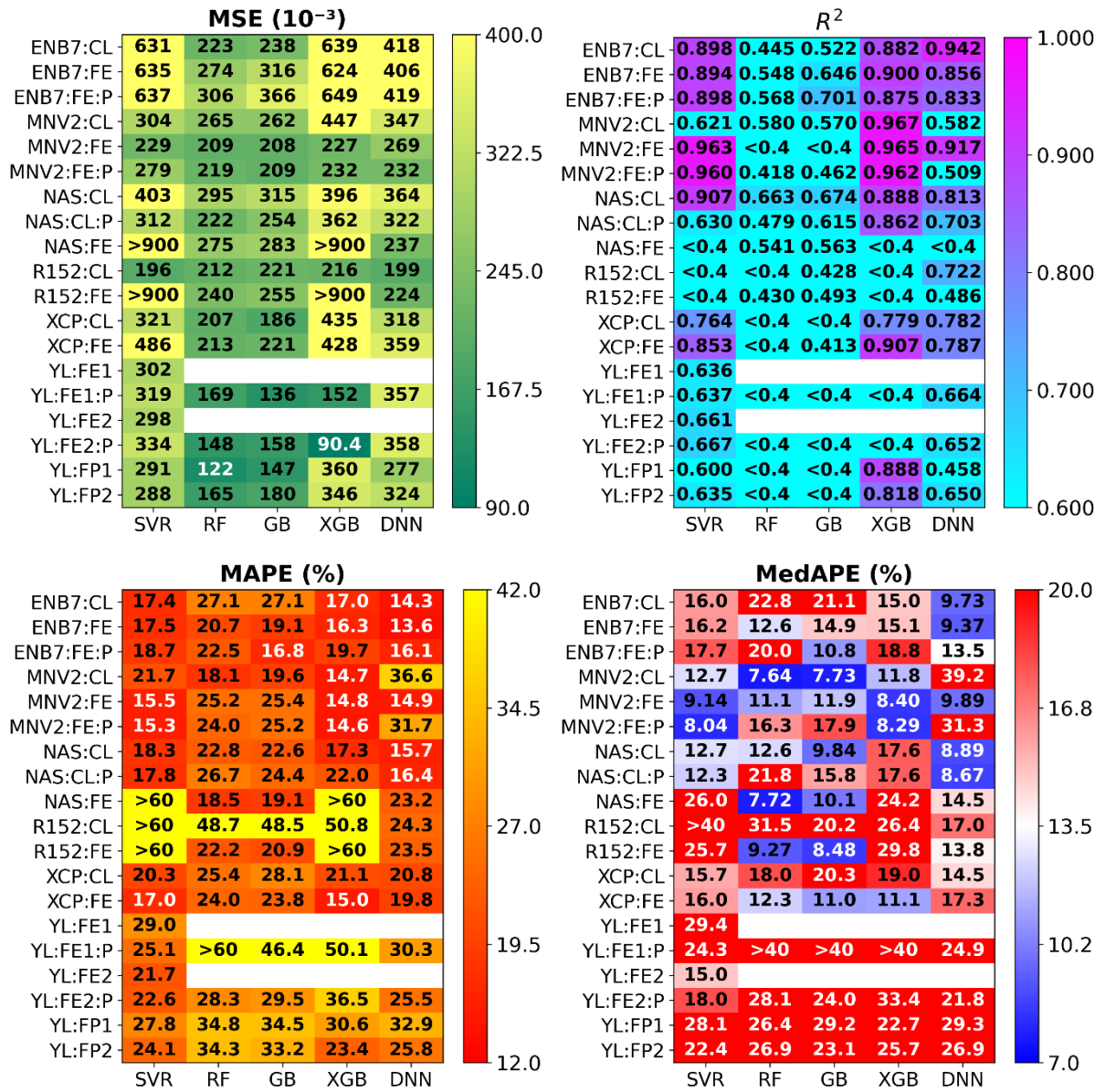
Fig. S6.5. Mean squared error, coefficient of determination, mean absolute percentage error, and median absolute percentage error for different combinations of computer vision models (vertical axis) and regression models (horizontal axis) during the test phase with experimental dataset with post-hoc calibration . The models were trained on a simulated dataset .
