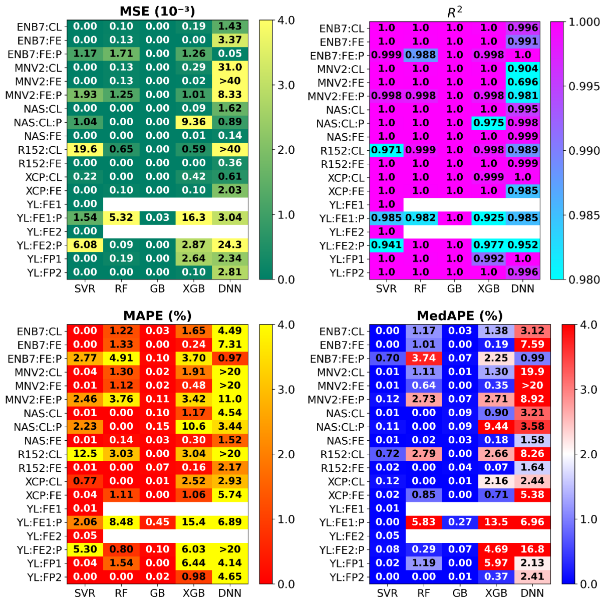
Fig. S6.7. Mean squared error, coefficient of determination, mean absolute percentage error, and median absolute percentage error for different combinations of computer vision models (vertical axis) and regression models (horizontal axis) during the training phase . The models were trained on an experimental dataset .
