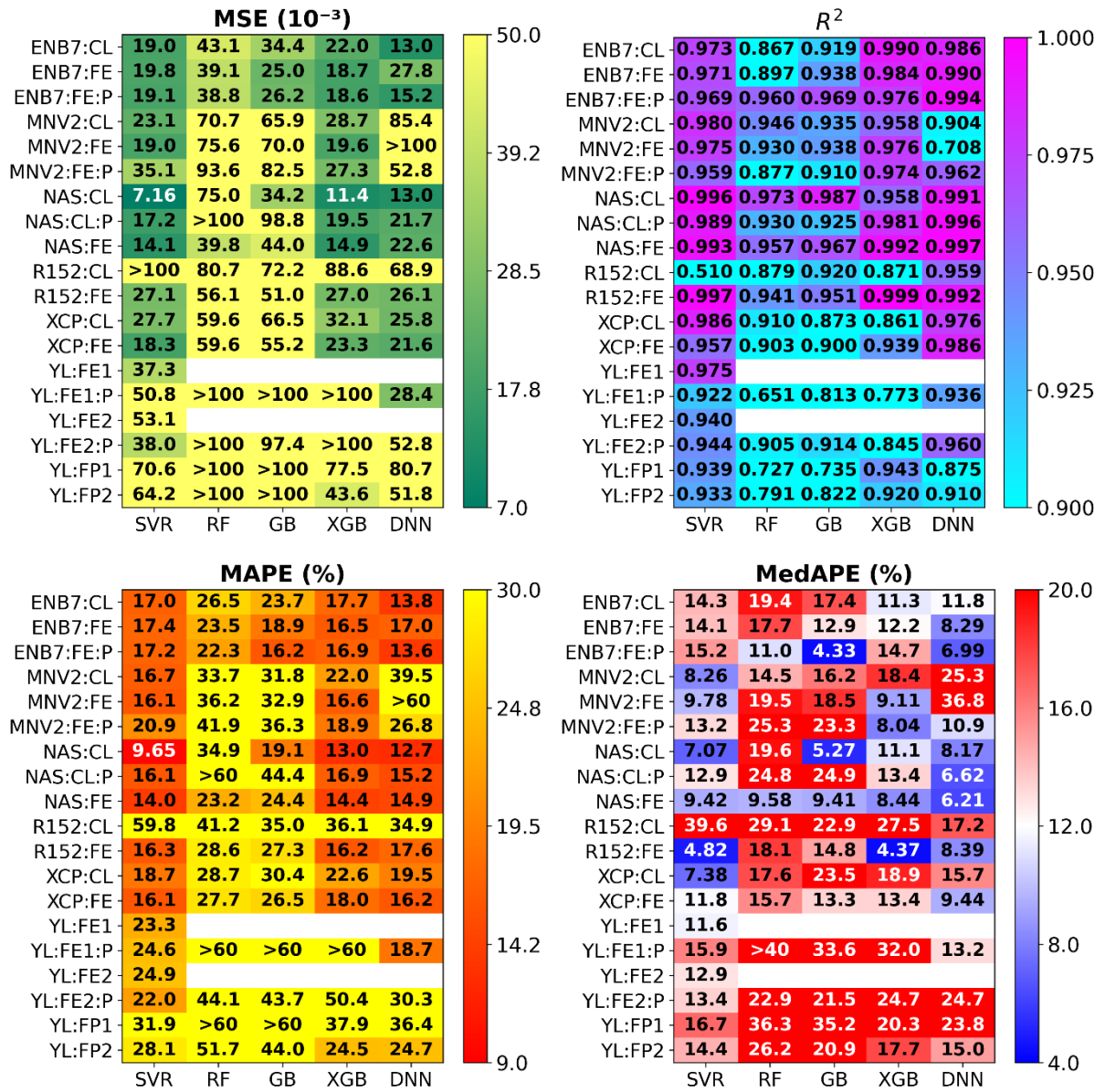
Fig. S6.8. Mean squared error, coefficient of determination, mean absolute percentage error, and median absolute percentage error for different combinations of computer vision models (vertical axis) and regression models (horizontal axis) during the test phase . The models were trained on an experimental dataset .
