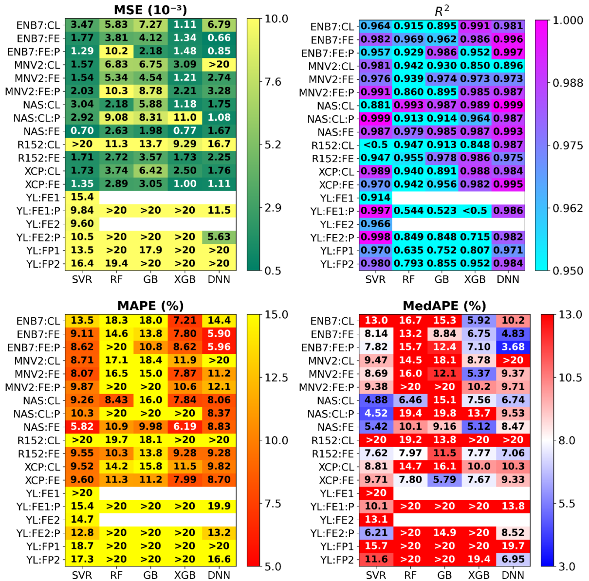
Fig. S6.3. Mean squared error, coefficient of determination, mean absolute percentage error, and median absolute percentage error for different combinations of computer vision models (vertical axis) and regression models (horizontal axis) during the test phase with simulated dataset. The models were trained on a simulated dataset .
