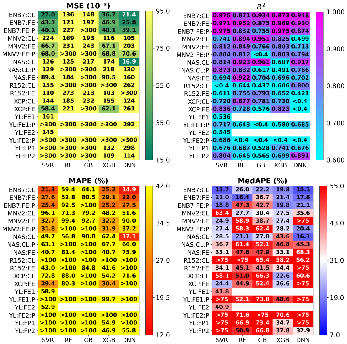
Fig. S6.4. Mean squared error, coefficient of determination, mean absolute percentage error, and median absolute percentage error for different combinations of computer vision models (vertical axis) and regression models (horizontal axis) during the test phase with experimental dataset without post-hoc calibration . The models were trained on a simulated dataset .
